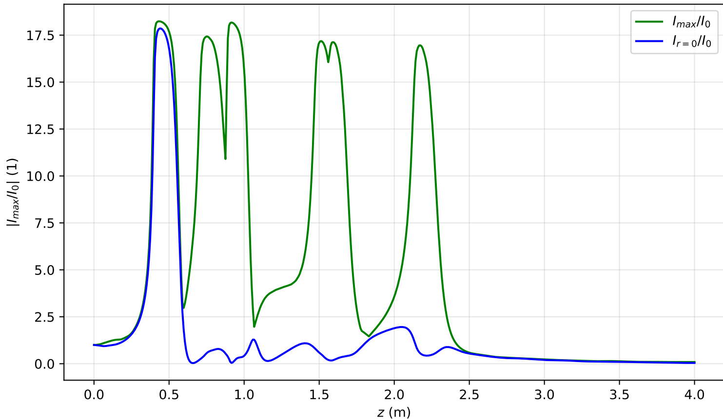
I_{\max}(x=0, y=0, z)/I_0 , \text{Pin}=6.1\text{Pcr} , noisy input, artificial time
